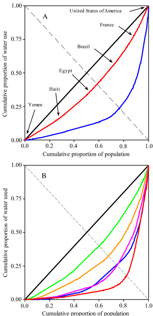
Figure 2. (A) Lorenz curves for total water footprint (red) and total renewable water resources (blue). The locations of water footprints for some representative countries are labeled within the bounds of this figure. The United States of America is at the upper extreme of the curve. Countries that fall between France and the United States include Canada and Portugal. Countries that fall toward the middle of the curve, for instance between Egypt and Brazil, include Japan and the United Kingdom. Countries at the lower end of the curve, between Yemen and Haiti, include Afghanistan and Ethiopia. (B) Lorenz curves for five water components of water use. The green Lorenz curve is for the internal agricultural water footprint. The orange Lorenz curve is for household uses water footprint. The blue Lorenz curve is for the internal industrial water footprint. The pink Lorenz curve is for the external agricultural water footprint. The red Lorenz curve is for the external industrial water footprint.
